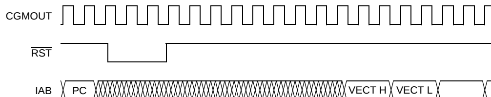
Figure 8-4. External Reset Timing
