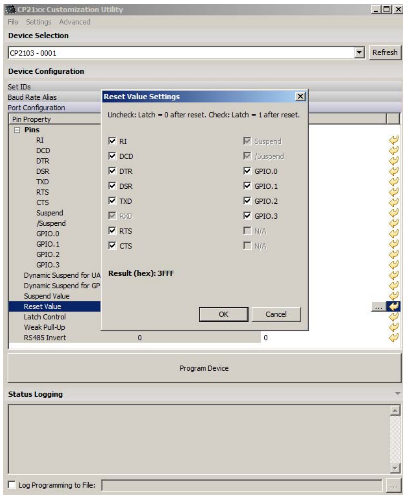
Figure 14. Latch Settings
