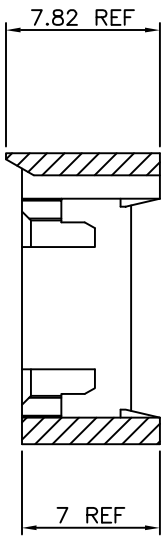
SECTION B-B
