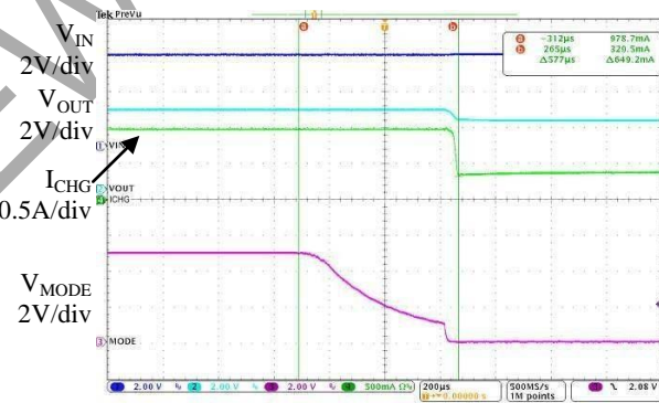
Time 200μs/div Figure 9. MODE Pin Pull Low
