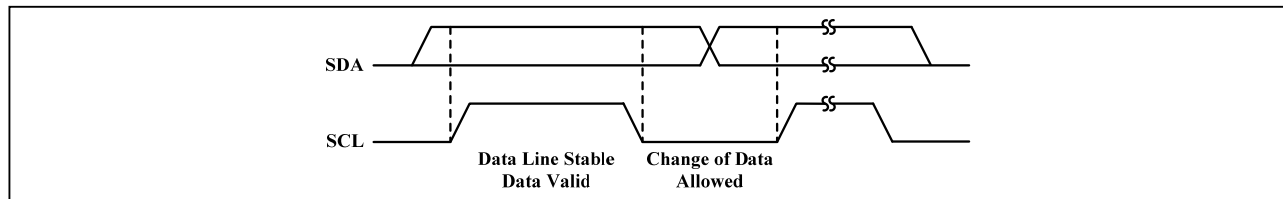
Figure 4 Bit Transfer
