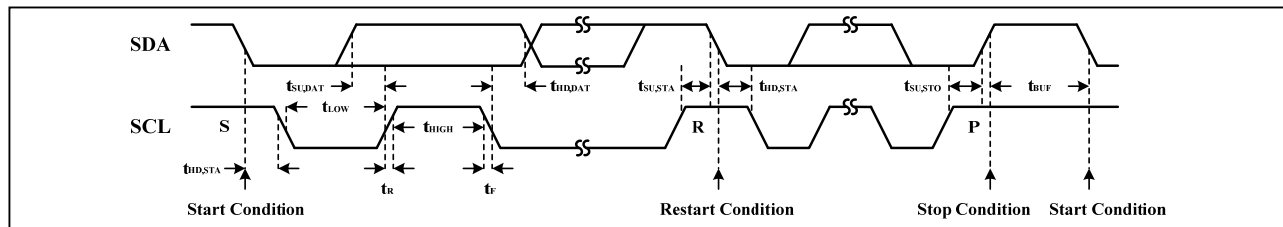
Figure 3 Interface Timing
