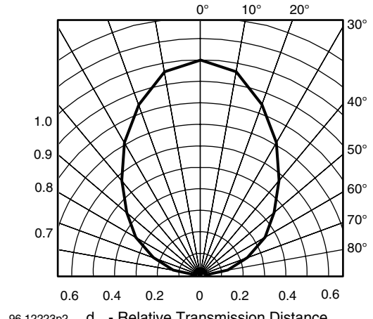
96 12223p2 d_{rel} - Relative Transmission Distance Fig. 12 - Horizontal Directivity
