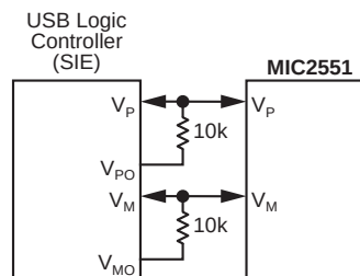
Figure 8. MIC2551 Interface to Non-Multiplexed Data Bus
