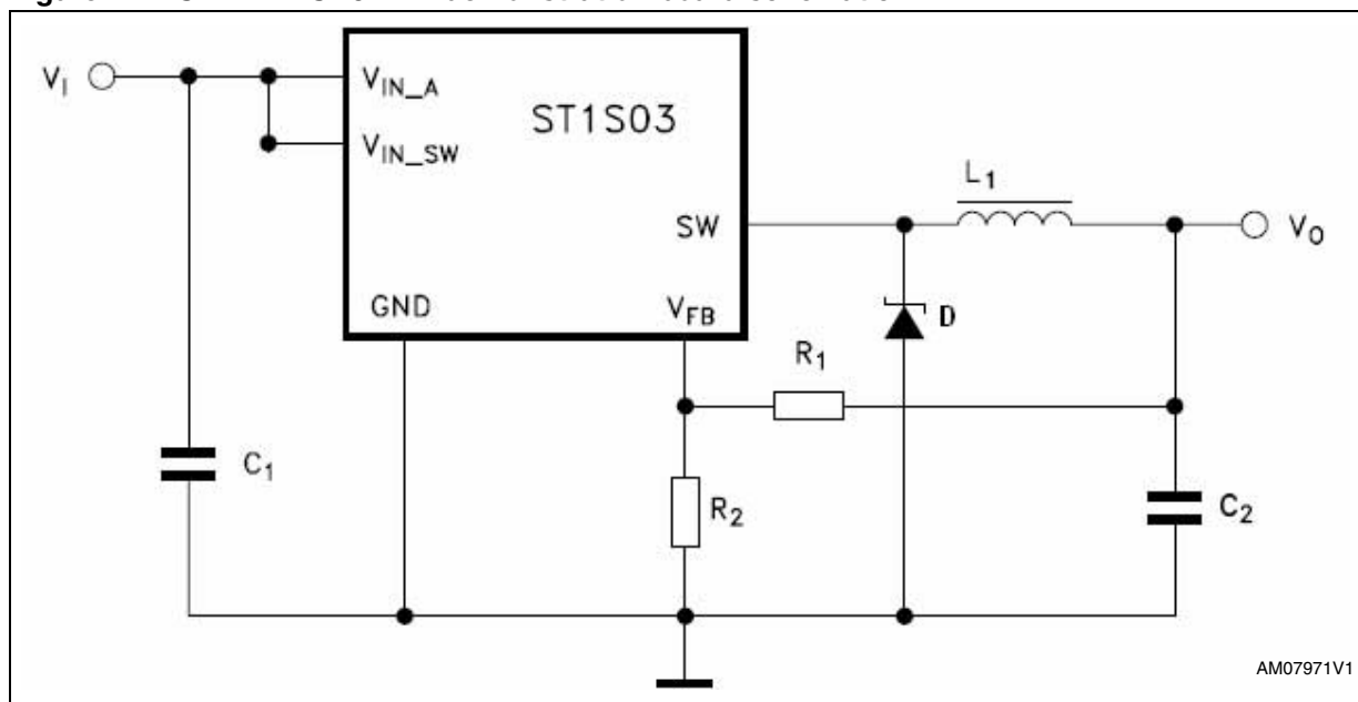
Figure 1. STEVAL-ISA042V2 demonstration board schematic
