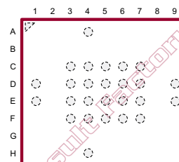
26-Ball fpBGA (top view)
