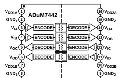
Figure 3. ADuM7442
