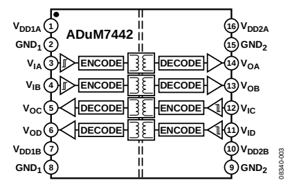
Figure 3. ADuM7442
