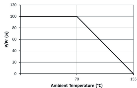
Derating Curve
