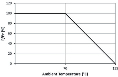
Derating Curve
