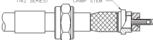
RG-58, RG-142 CABLE GROUP (142 SERIES)
