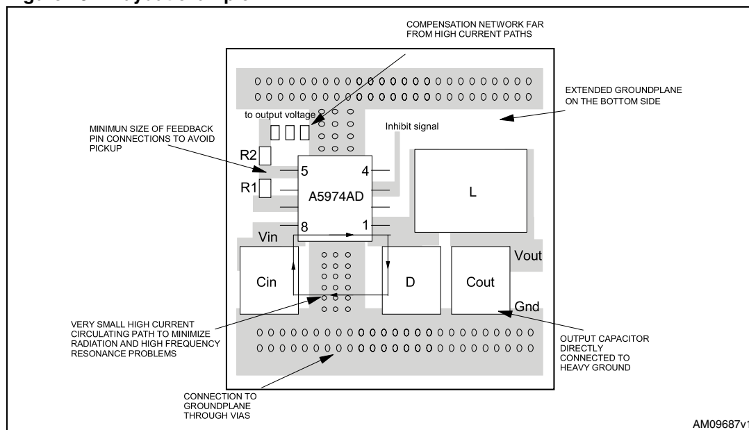
Figure 13. Layout example
