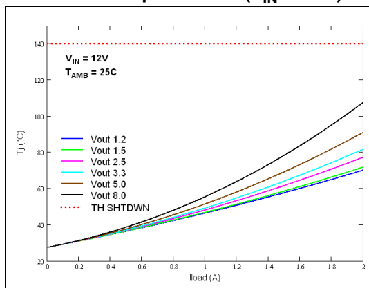
Figure 36. Junction temperature vs. output current ( V_{IN} = 12V )
