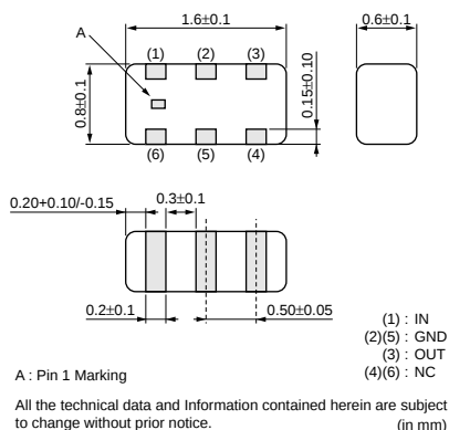
LFL18_TC1 Series
