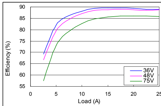
Fig. 2 Typical efficiency of AVO75-48S1V5
