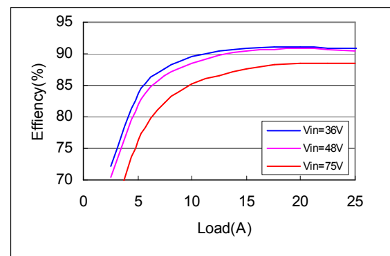
Fig. 4 Typical efficiency of AVO75-48S2V5
