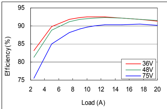
Fig. 5 Typical efficiency of AVO75-48S3V3
