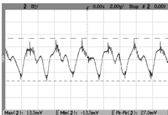
Fig. 50 Typical output ripple voltage of AVO75-48S1V2 room temperature, I_o=I_{o,max}
