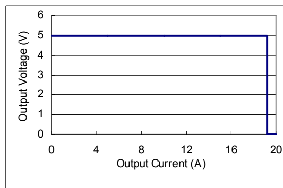
Fig. 13 Typical output over-current of AVO75-48S05
