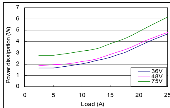
Fig. 16 Typical power dissipation of AVO75-48S1V5
