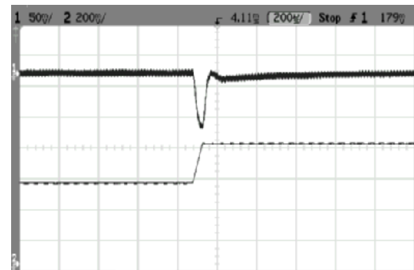
Fig. 39 AVO75-48S3V3 typical transient response to step increase in load from 50% to 75% of full load, room temperature, 48Vdc input ( \Delta I_o/\Delta t=0.1A/1\mu s )
