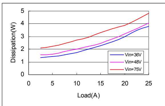
Fig. 15 Typical power dissipation of AVO75-48S1V2
