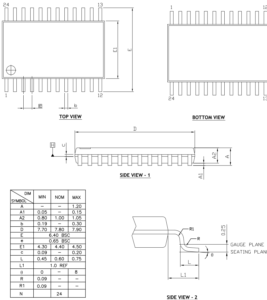
TERMINAL DETAILS
