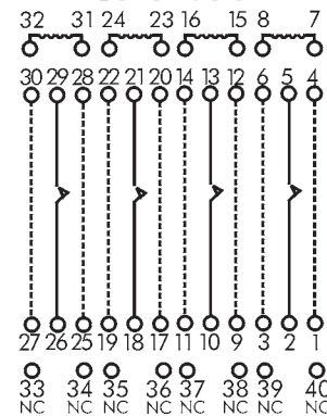
Top View Schematic
