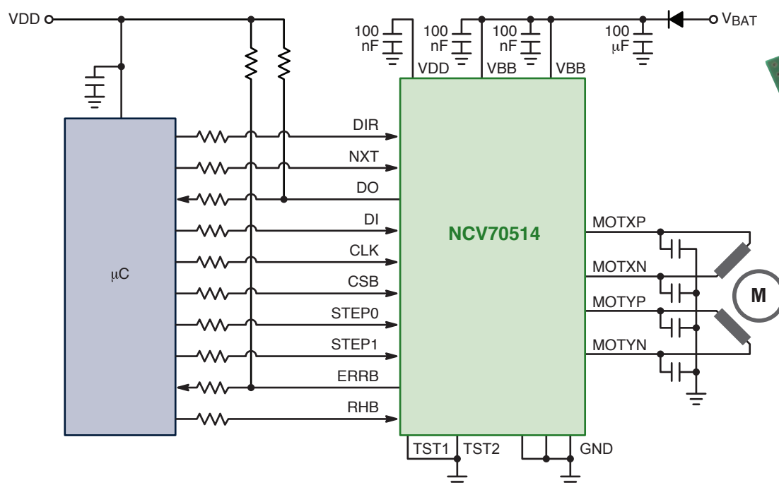
Evaluation Board NV705143R1DBGEBB
