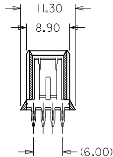
SECTION: Y-Y
