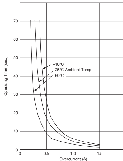
PTGL10BB120N0P52A0
