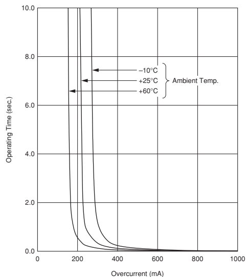
PRG18BC6R8MM1RB
