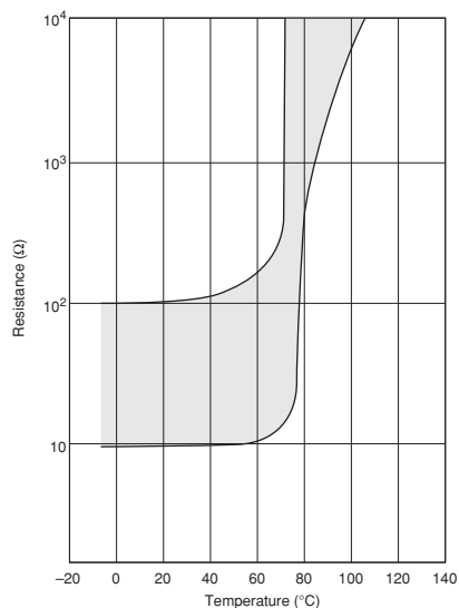
PTF_04BF471Q2N34B0
