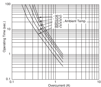
PTGL07AS150K6B51B0
