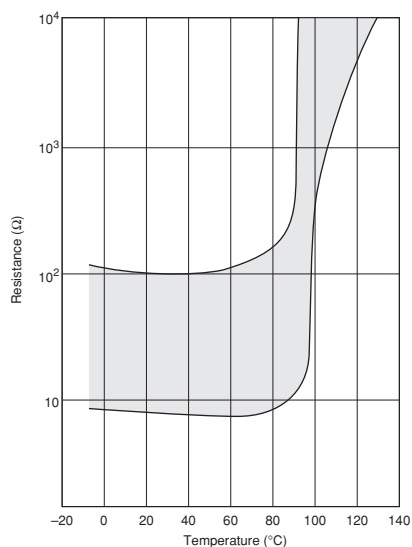
PTF_04BD471Q2N34B0
