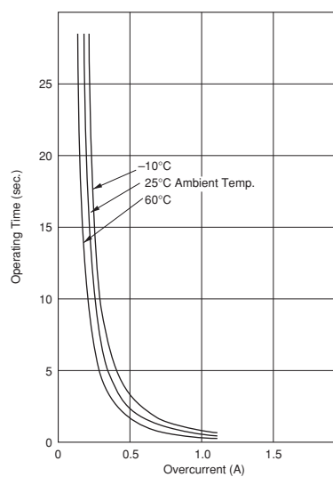
PTGL07AR560M9A51B0
