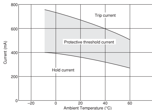
PTGL12AR5R6H4B71B0
