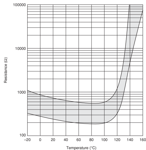
PRF18/21AR471Q Type
