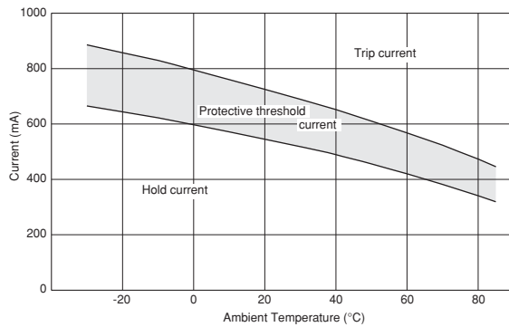
PTGL07AS1R8K2B51B0
