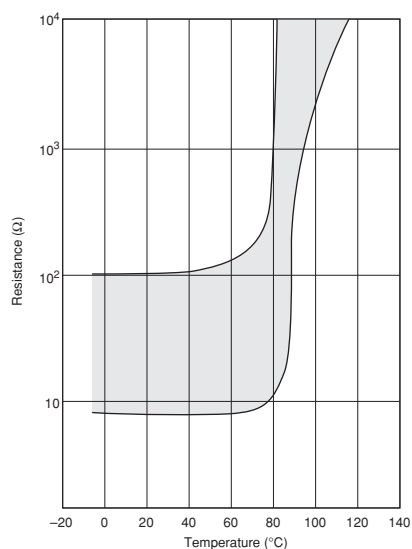
PTF_04BE471Q2N34B0
