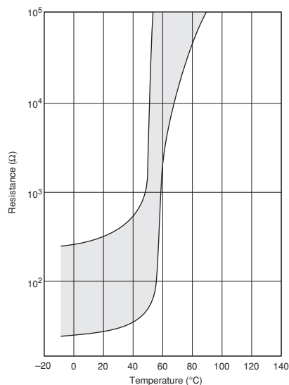
PTF_04BH222Q2N34B0
