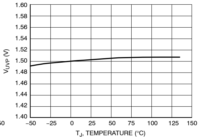
Figure 20. Output Under Voltage Level versus Temperature (Fault Mode Options A & B)
