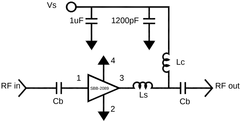
Application Schematic
