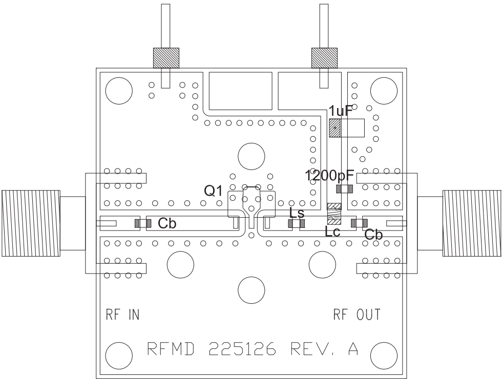
Evaluation Board Layout
