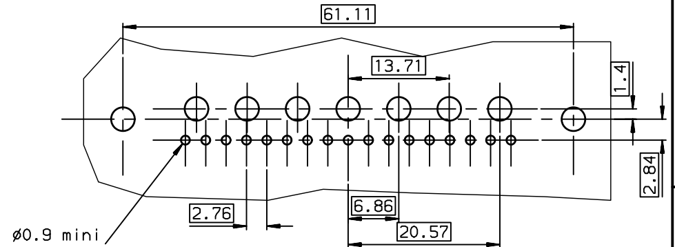
LAYOUT DIMENSIONS (after plating) CONNECTOR SIDE VIEW
