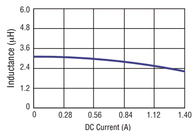
SRN3010TA-3R3M
