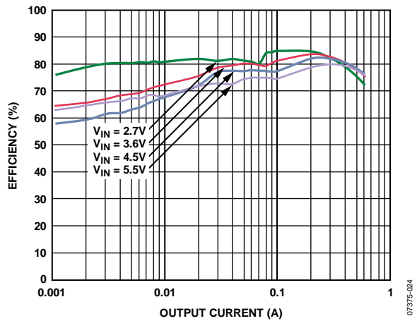
Figure 14. Efficiency, V_{OUT} = 1.0 V
