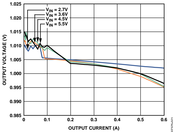
Figure 11. Load Regulation, V_{OUT} = 1.0 V
