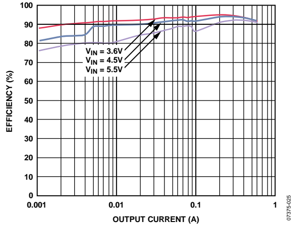
Figure 15. Efficiency, V_{OUT} = 3.3 V
