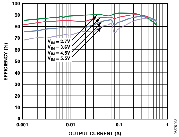
Figure 13. Efficiency, V_{OUT} = 1.8 V
