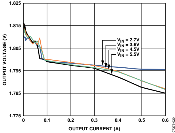
Figure 10. Load Regulation, V_{OUT} = 1.8 V
