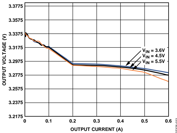
Figure 12. Load Regulation, V_{OUT} = 3.3 V
