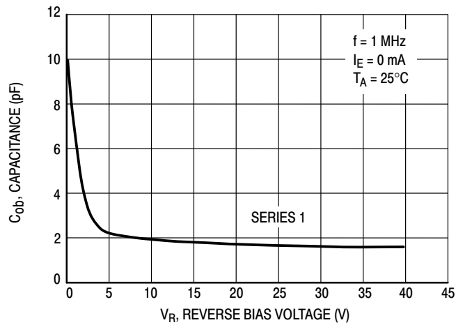
Figure 30. Output Capacitance
