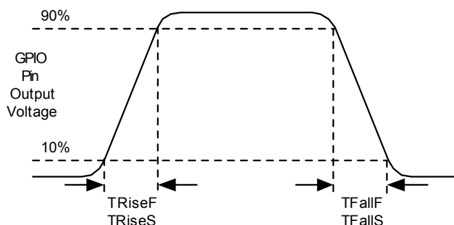
Figure 6. GPIO Timing Diagram
