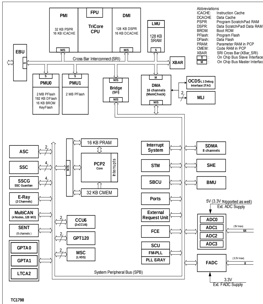
Figure 1 Block Diagram
