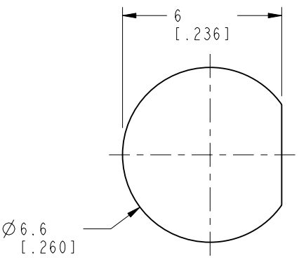
SCALE 5.000 RECOMMENDED MOUNTING HOLE DIMENSIONS
