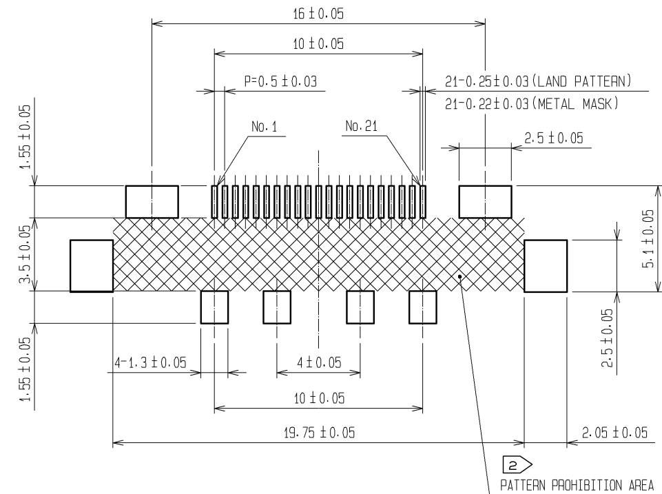
RECOMMENDED LAND PATTERN DIMENSION (4:1)
