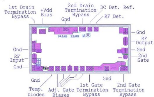
40MHz - 30GHz bonding diagram
