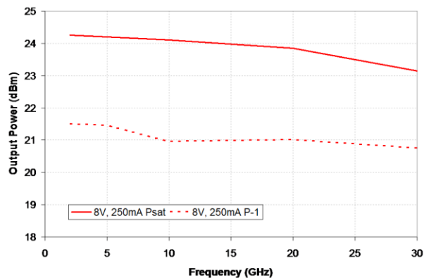
Output Power
