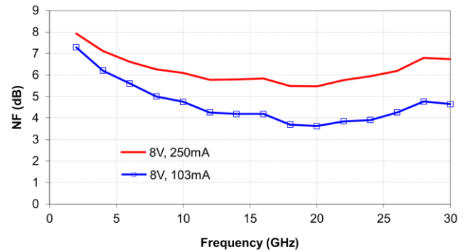
Noise Figure
