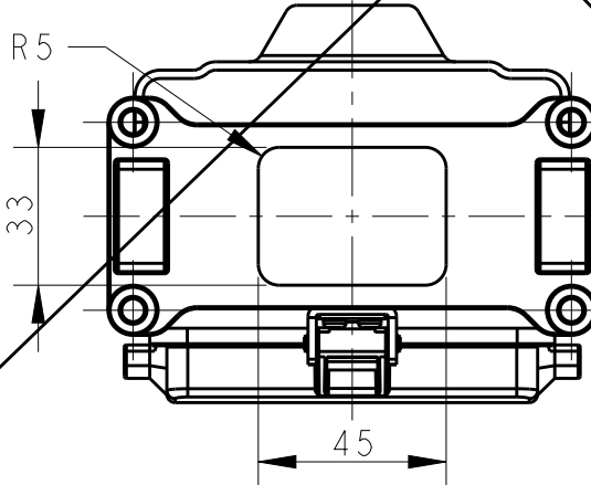
HOUSING 下壳
