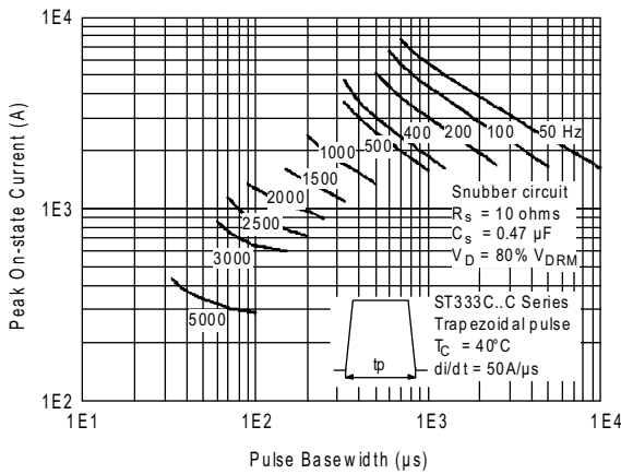
Fig. 14 - Frequency Characteristics
