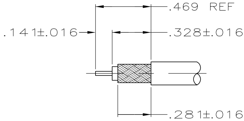
RECOMMENDED STRIP LENGTH SCALE: 2:1
