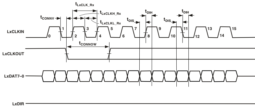
Figure 18. Link Ports—Receive
