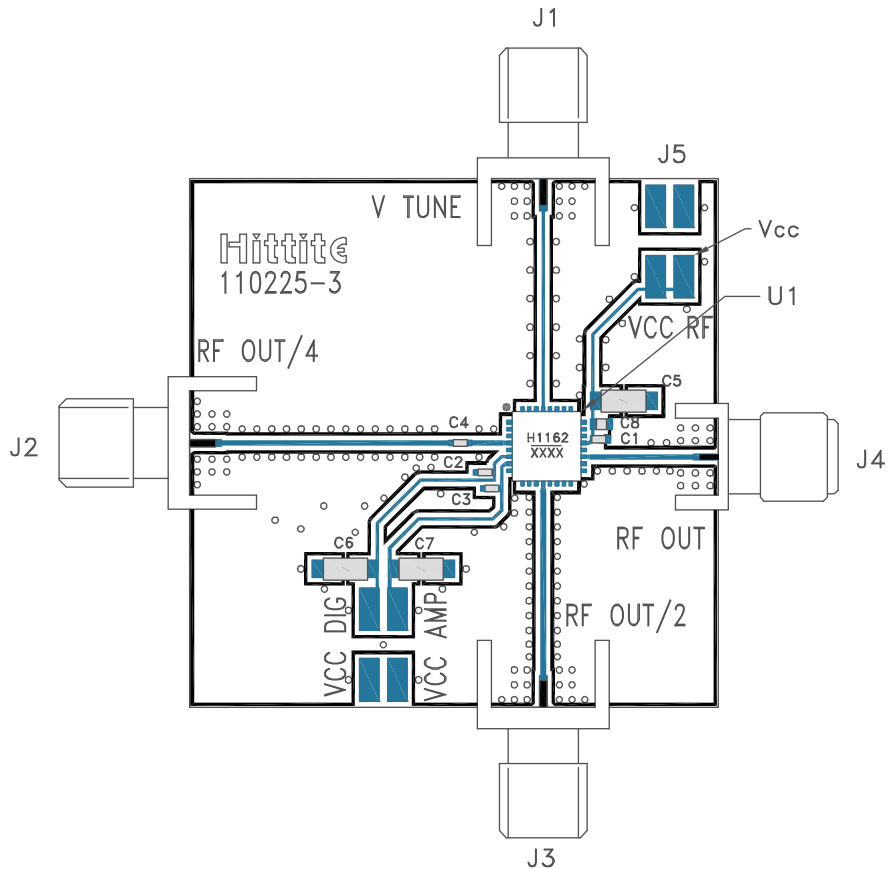
Figure 17. Evaluation Board
