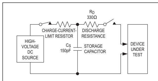
Figure 47. IEC 61000-4-2 Contact Discharge ESD Test Circuit
