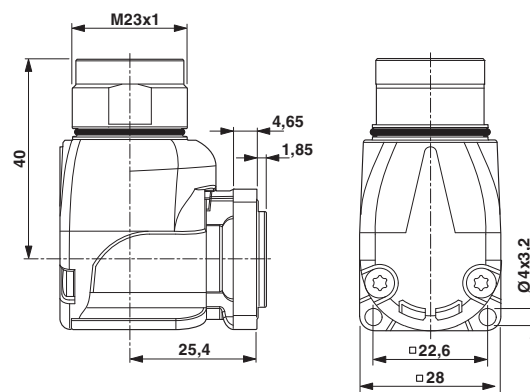
Dimensioned drawing
