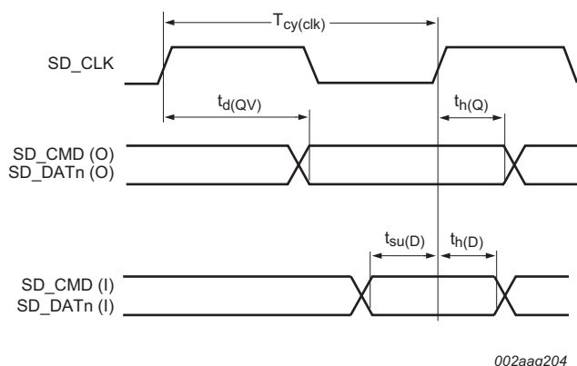
Fig 40. SD/MMC timing
