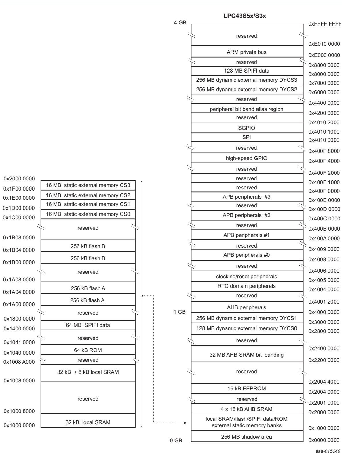
Fig 7. LPC43S5x/S3x Memory mapping (overview)
