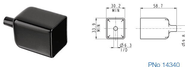
Insulation Boot
