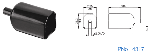
Insulation Boot
