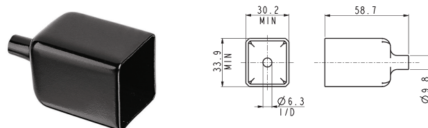
Insulation Boot
