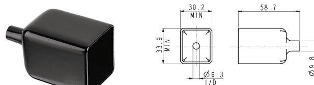
Insulation Boot
