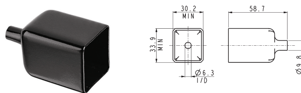
Insulation Boot
