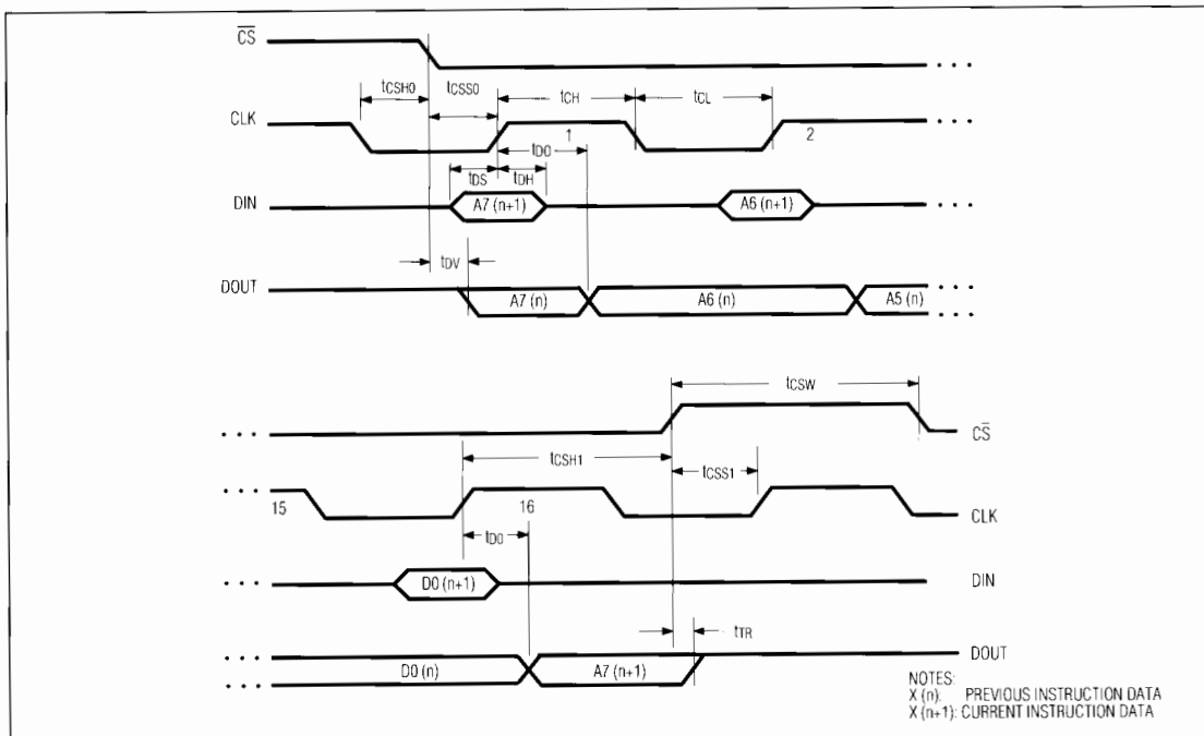
Figure 5. Timing Diagram
