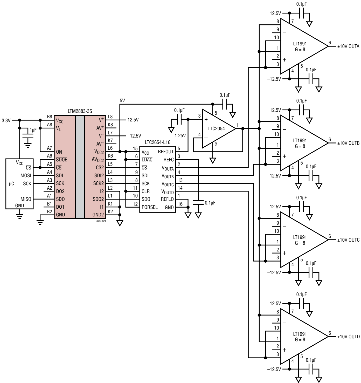
Figure 21. Quad 16-Bit \pm 10V Output Range DAC
