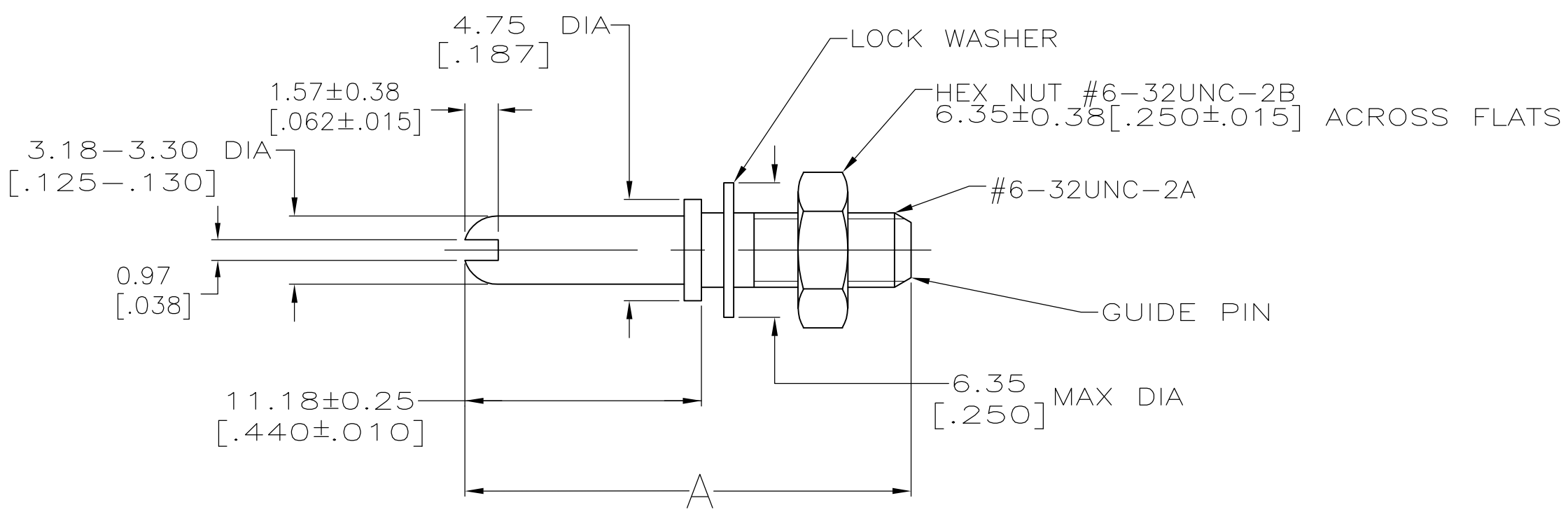
ASSEMBLED VIEW
