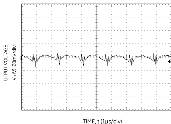
Figure 3. Typical output ripple and noise ( C_o=10\mu\text{F} ceramic, V_{IN} = 8\text{V} , I_o = I_{o,max} ).
