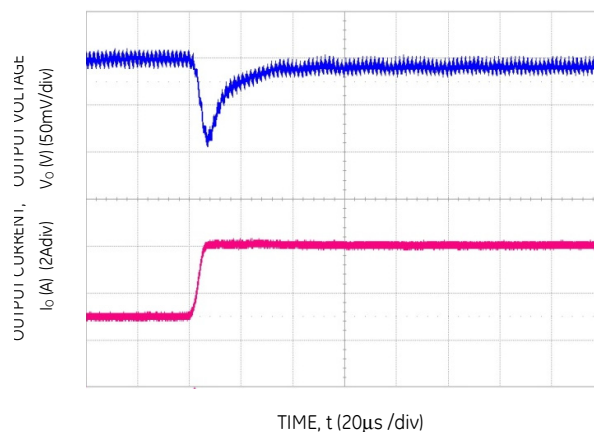
Figure 34. Transient Response to Dynamic Load Change from 50% to 100% at 12Vin, C_{out}=2\times 47\mu\text{F} , C_{Tune}=2200\text{pF} & R_{Tune}=261
