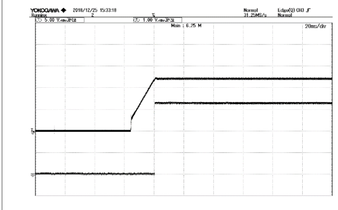
Figure 9: PG voltage vs. Vout @ Vin=220Vac, 0A out TOP: Vout, 5V/div, 20mS/div BOTTOM: PG, 1V/div, 20mS/div
